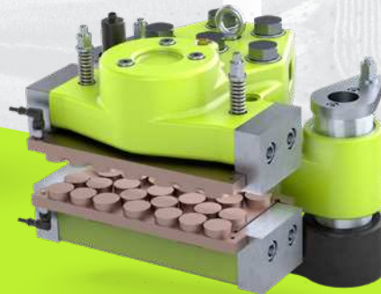
SFRA 8 WIND TURBINE BRAKES
