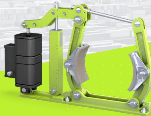
EBN 400 DRUM & BAND BRAKES
